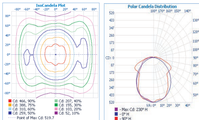
BS100LED-A-4HT120-277V
