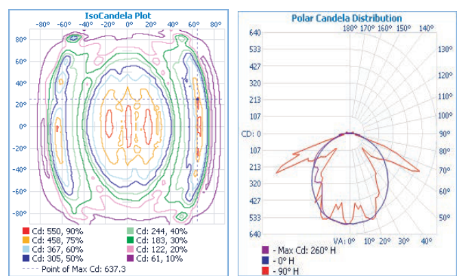
BS100LED-A-4HT120-277V-CL
